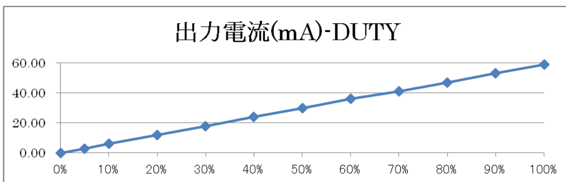
LEDVCC:12V PWM:1KHz 設定電流:59.46mA
