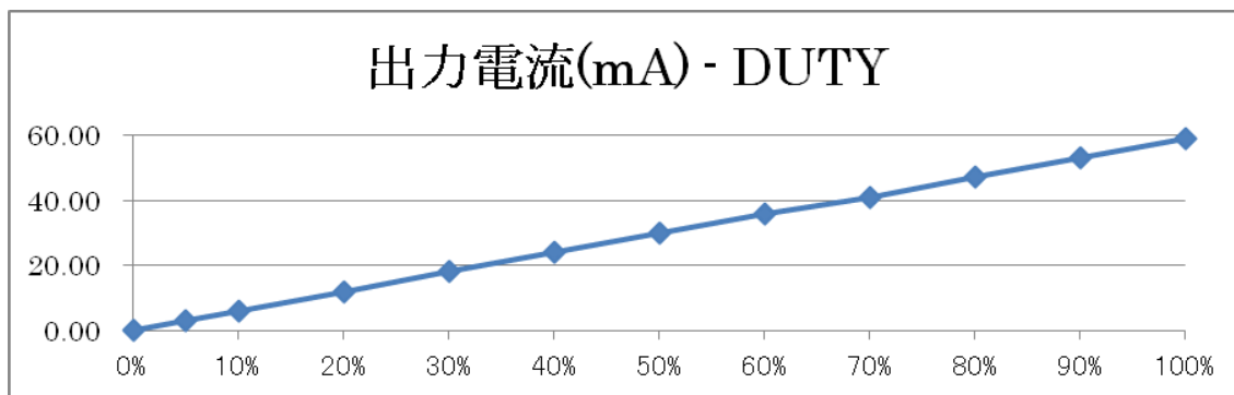
LEDVCC:5V PWM:1KHz 設定電流:59.46mA
