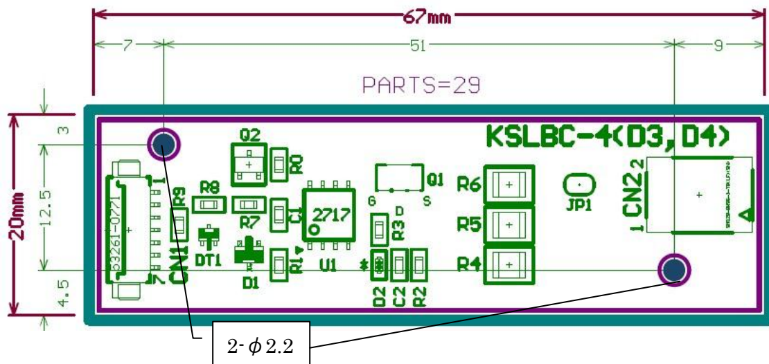
Substrate Dimensional Drawing for KSLBC-4 (D3, D4)
